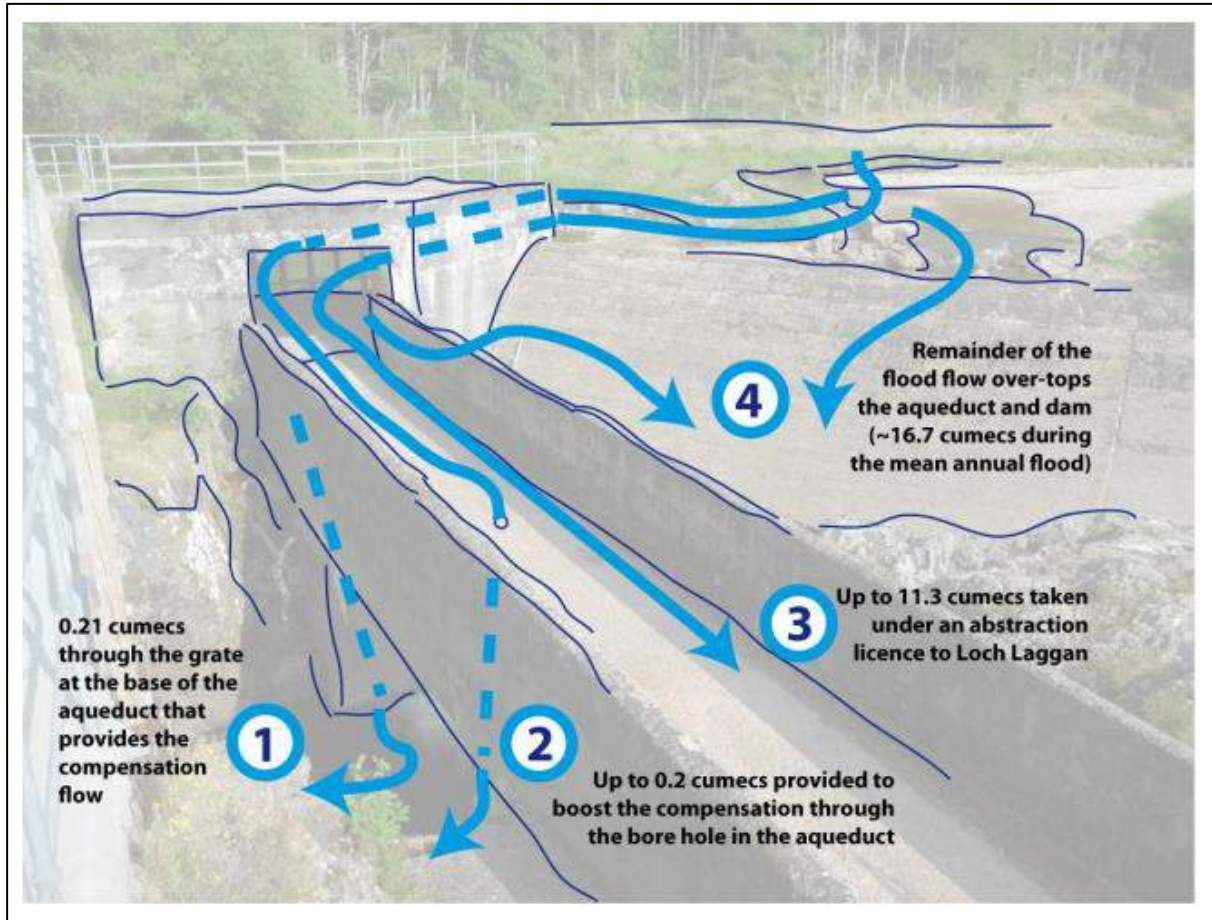
Figure 4-1: Schematic of Mashie Dam taken from CRESS Study (2010)
